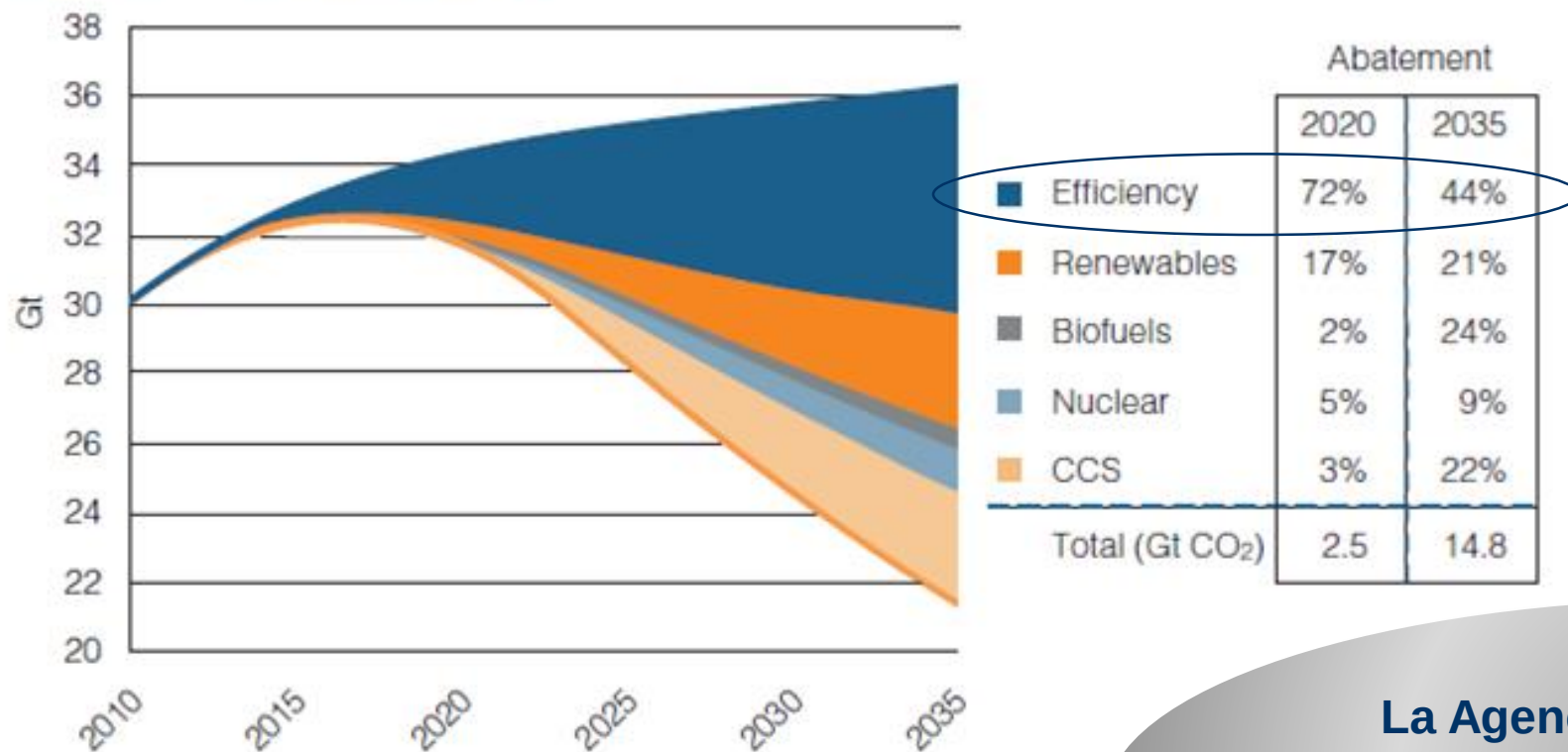
Scenarios for CO 2 emissions [3]
